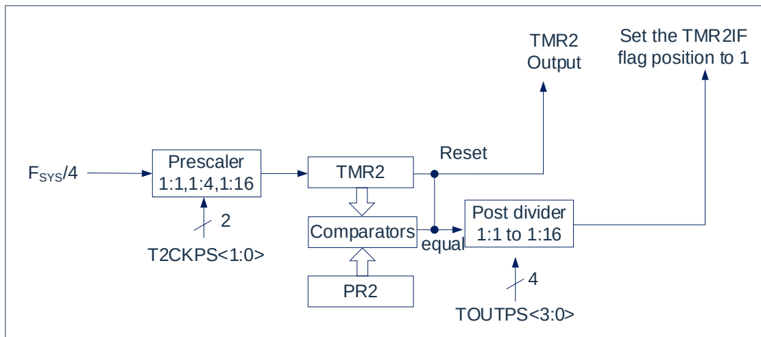
Fig 10-1: TIMER2 structure
