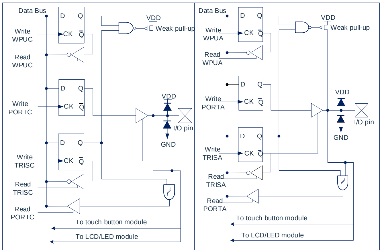
Fig 6-1: I/Oport structure (1)
