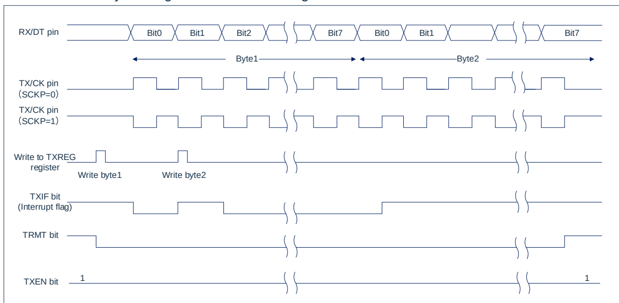
Fig 14-6: synchronous transmit
