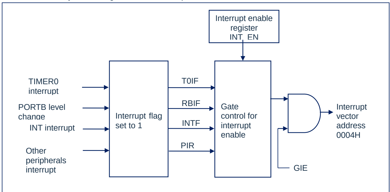
Fig 7-1: interrupt theory
